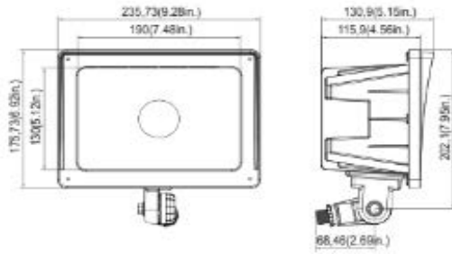
Knuckle Mount(35W&45W&65W)
