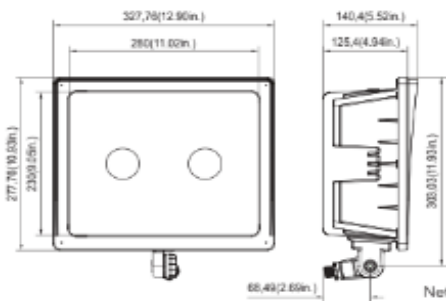
Knuckle Mount(70W&90W&110W)
