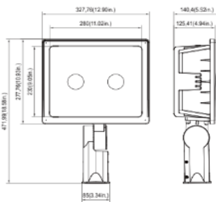
Slipfitter Mount(70W&90W&110W)
