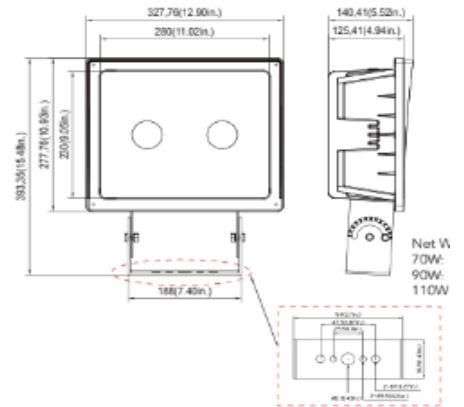
Trunnion Mount(70W&90W&110W)
