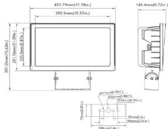
Trunnion Mount(140W&200W)
