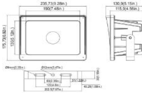
Trunnion Mount(35W&45W&65W)
