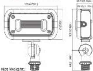
15W( Knuckle Mount)
