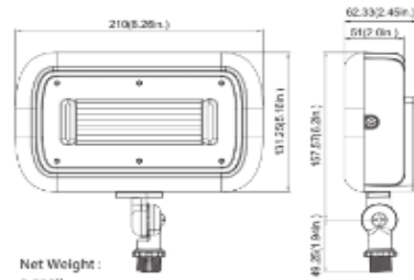
45W( Knuckle Mount)
