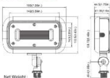
30W( Knuckle Mount)
