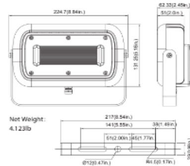
45W( Trunnion Mount)
