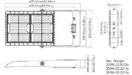
Trunnion Mount(250W&300W&350W)
