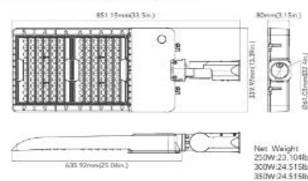
Slipfitter Mount(250W&300W&350W)
