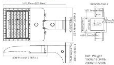
Wall Mount(150W&200W)
