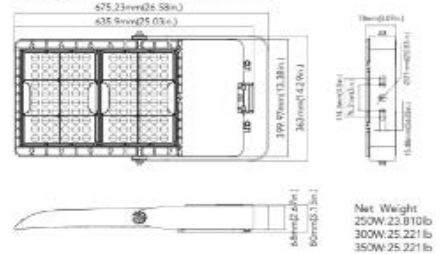
Trunnion Mount(250W&300W&350W)
