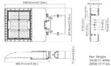
Yoke Mount(150W&200W)
