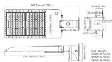
Wall Mount(250W&300W&350W)
