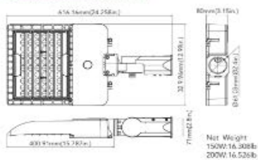
Slipfitter Mount(150W&200W)
